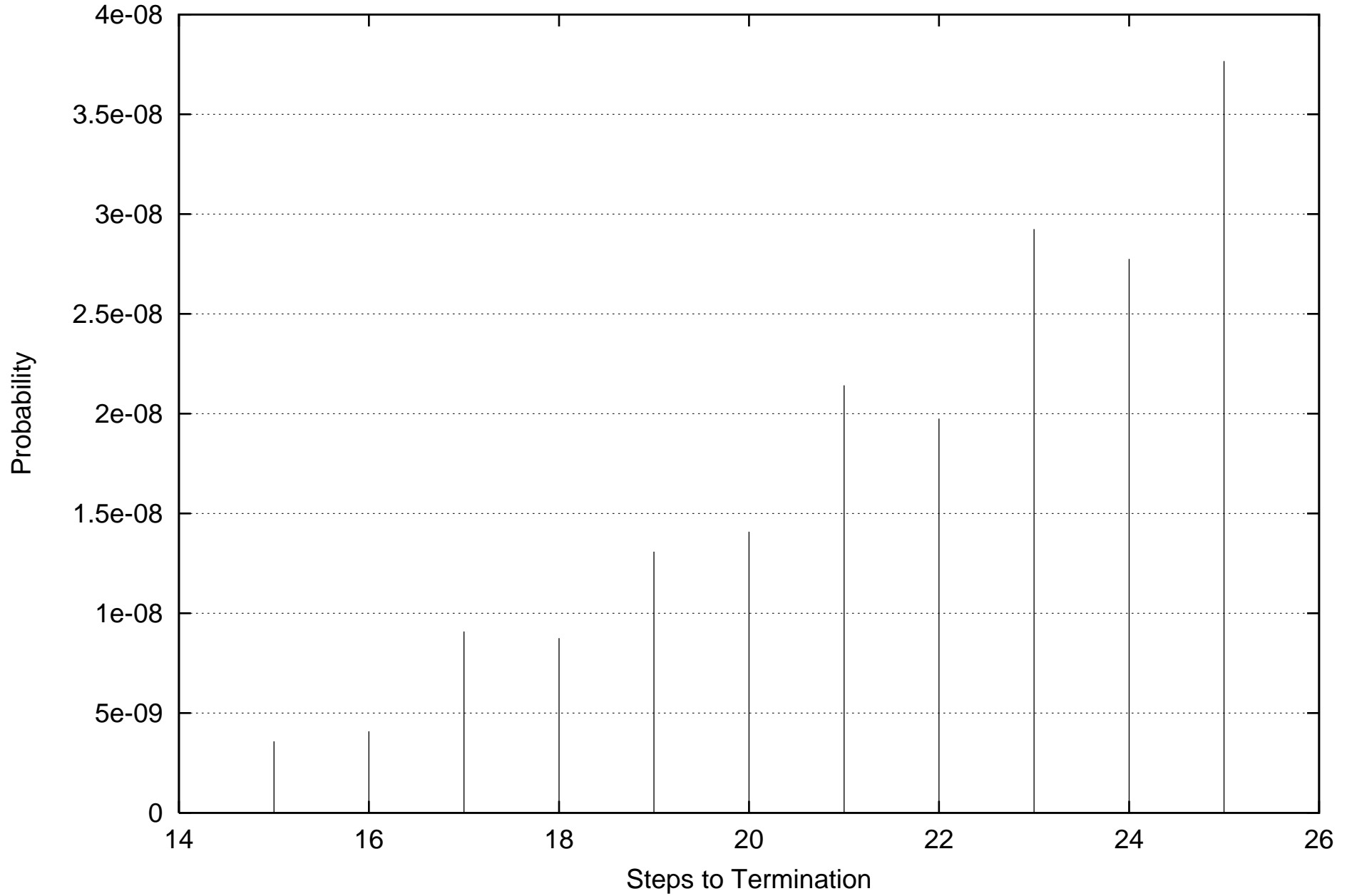
Self Trapping Random Walk on 4-D Lattice
