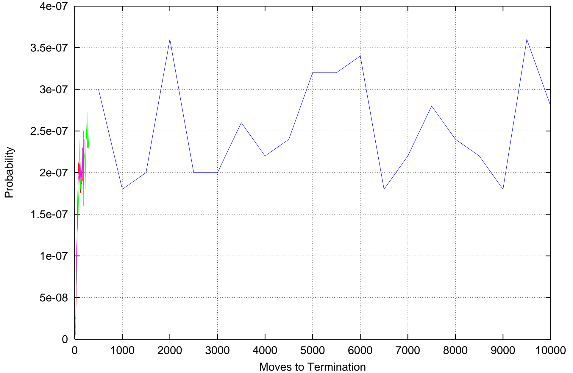
Self-Trapping Random Walk on 4-D Lattice
