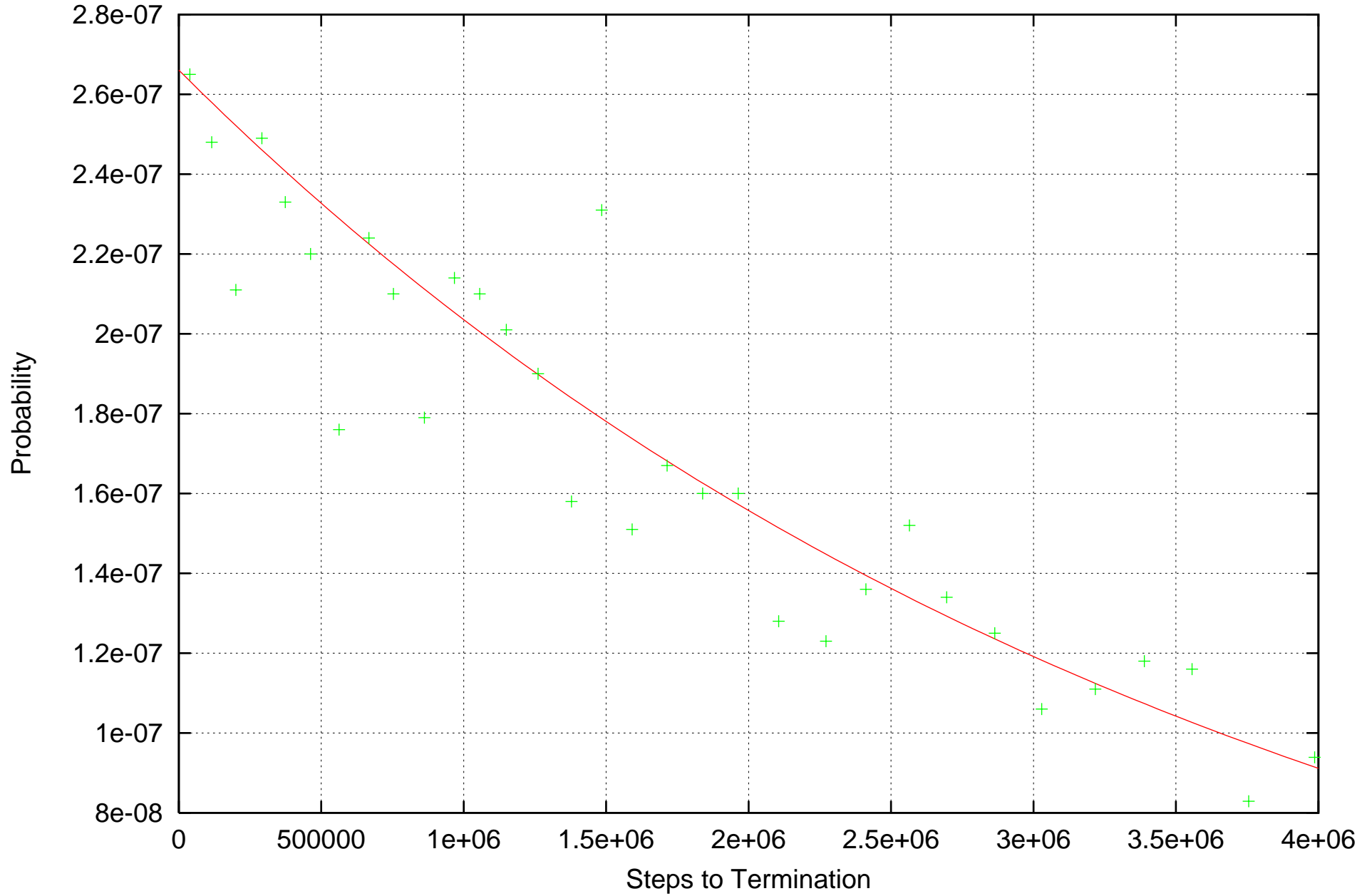
Self-Trapping Random Walk on 4-d Lattice ( 377^{**4} )
