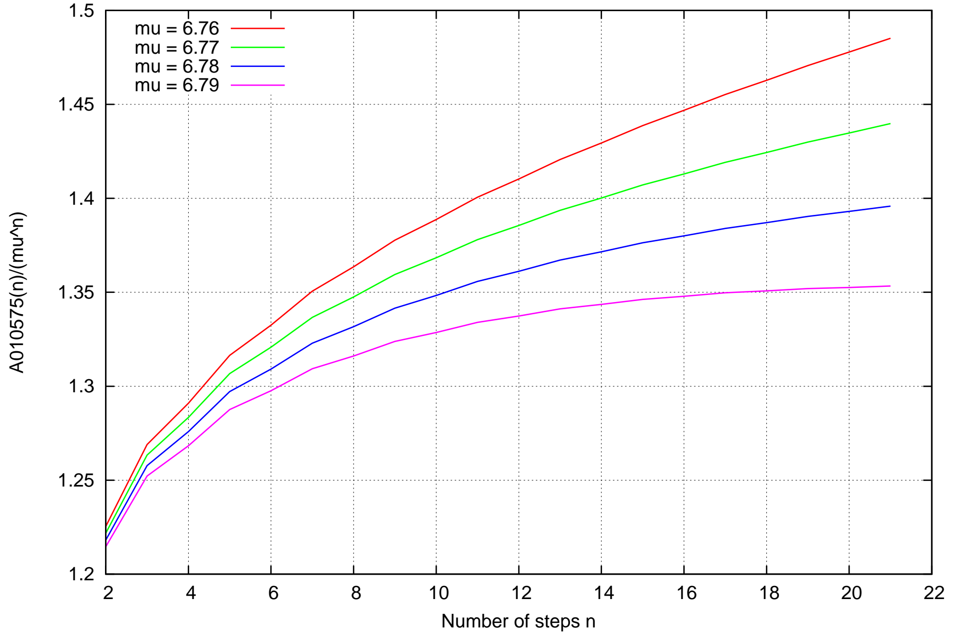
Asymptotic Behavior of Number of Self-Avoiding Walks on Z4
